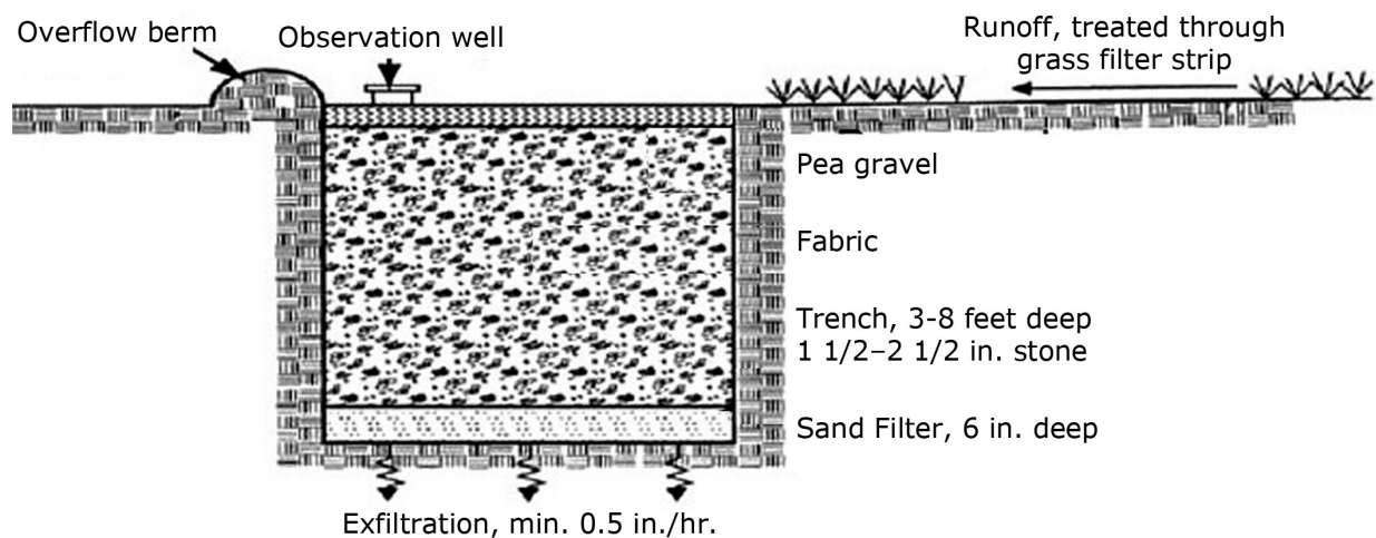
Figure 2. Profile view of typical infiltration practice (VA-DCR 2011).
